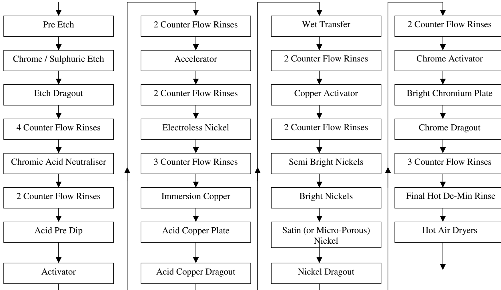
PLATING PLANT PROCESS MAP (CHART 1)
