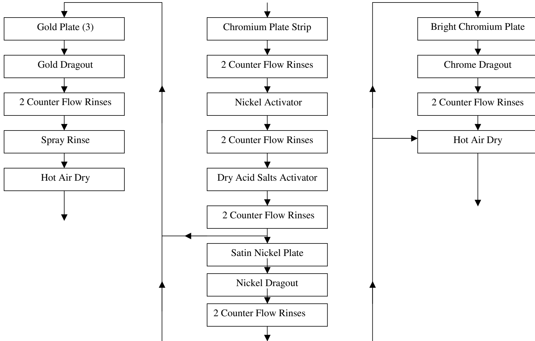
PLATING PLANT PROCESS MAP (CHART 2)
